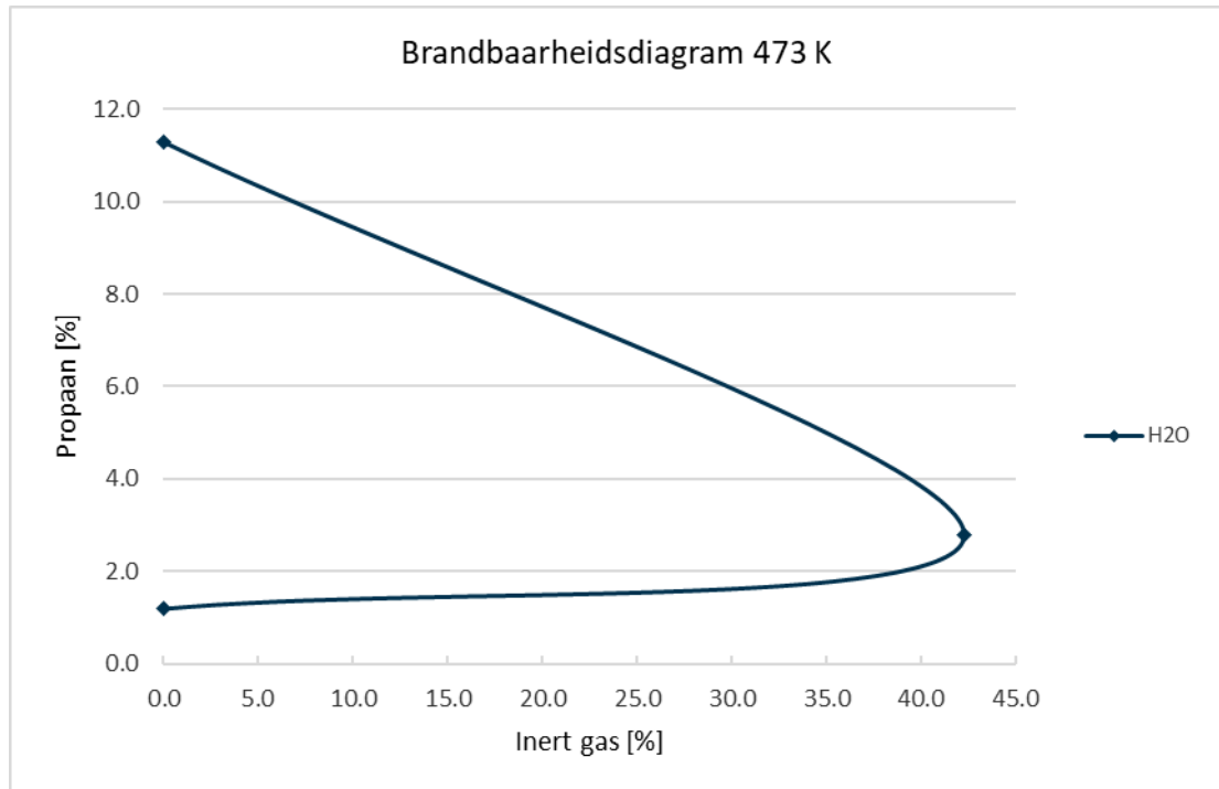
Figure 7: Flammability diagram for 473 K
