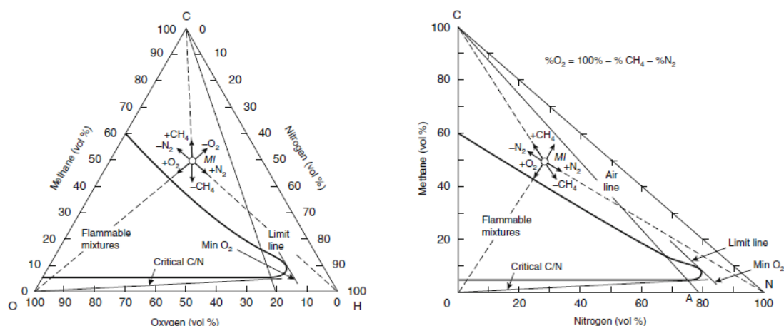
Figure 2: Flammability diagrams
