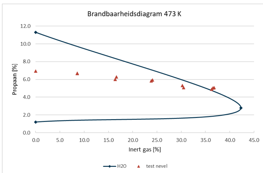
Figure 37: Flammability diagram for 473 K
