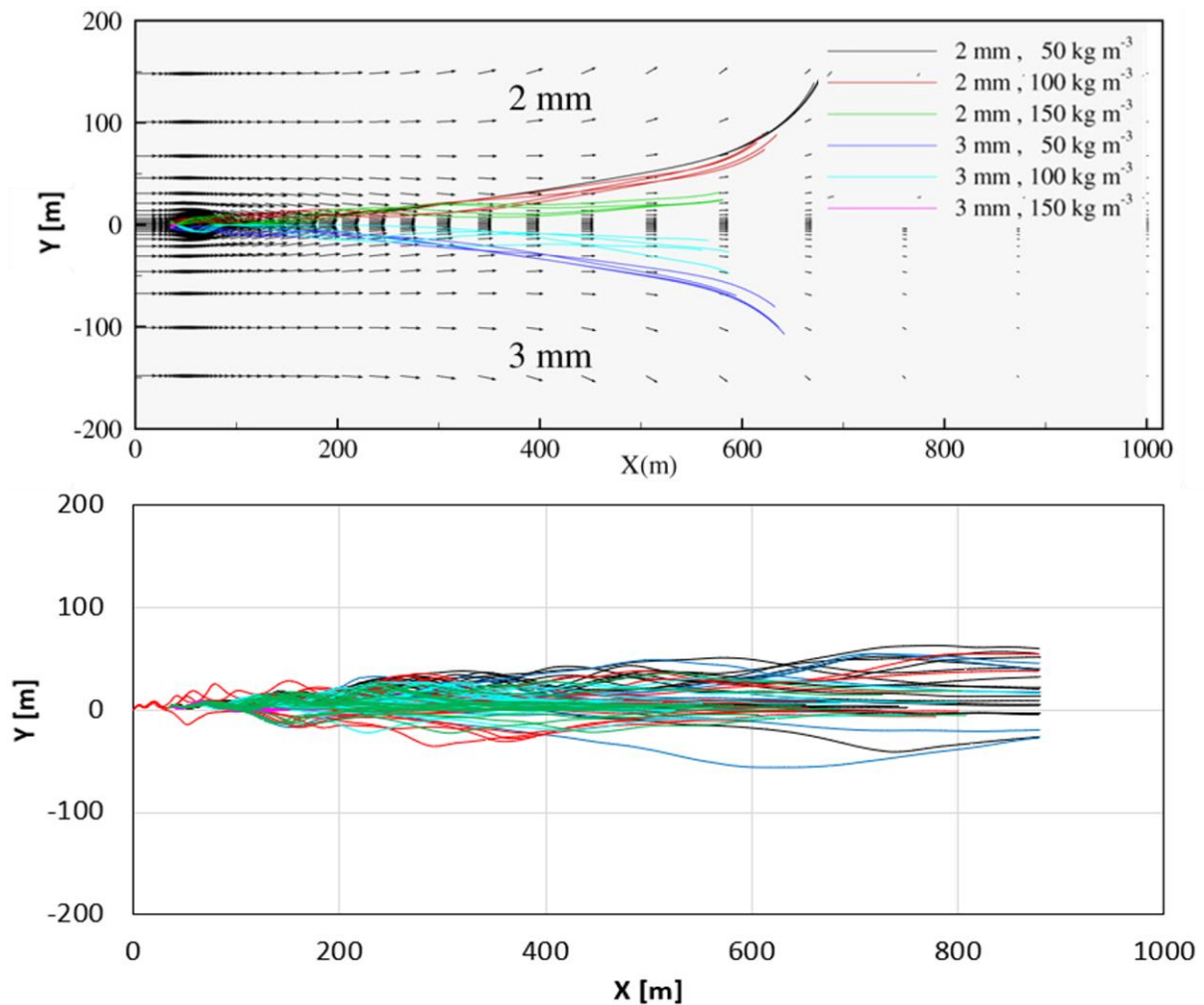
Figure 40: Firebrand trajectories in the horizontal plane as reported by Sardoy et al. [39] (top) and obtained from FDS simulations (bottom).
